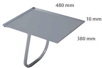
ARBETSBORD / WORK TABLE Article no. 800123
