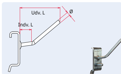
Topholder
