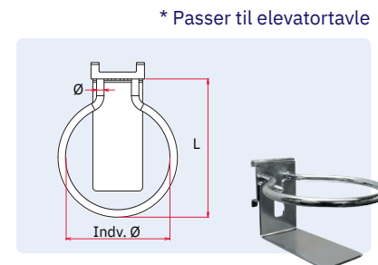
Spraydåseholder monteres i 4 huller
