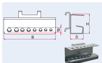
Borholder, monteres i 4 huller
